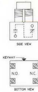
Typical Arrangement (Standard M1G1 shown) Figure 1
