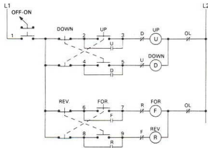
Typical Schematic Diagram Figure 4
