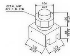
Approximate Dimensions Pushbutton Insert Figure 2
